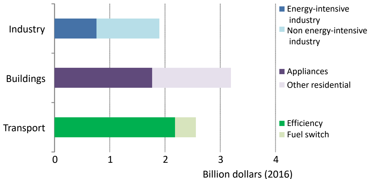
Average annual additional investment to 2030 in end-use sectors in the Sustainable Development Scenario
