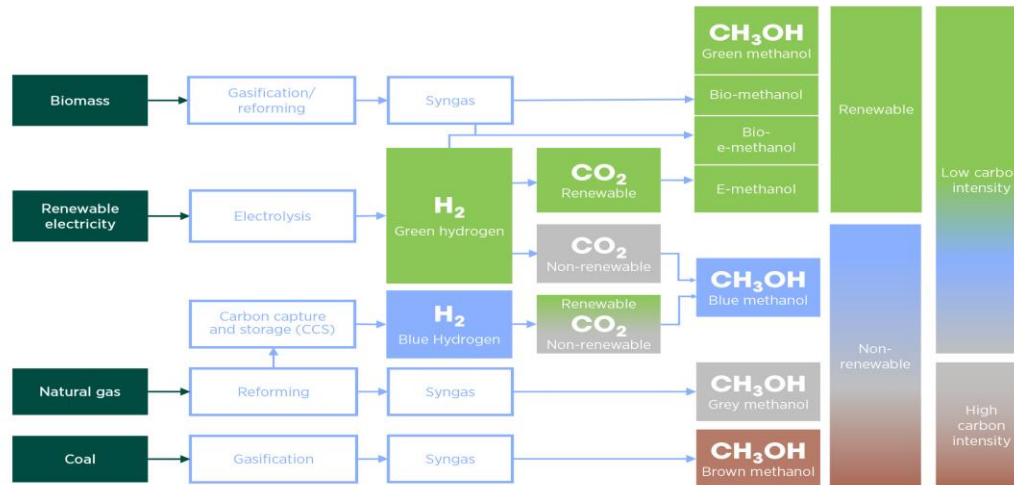
Figure 2. Principal methanol production routes
