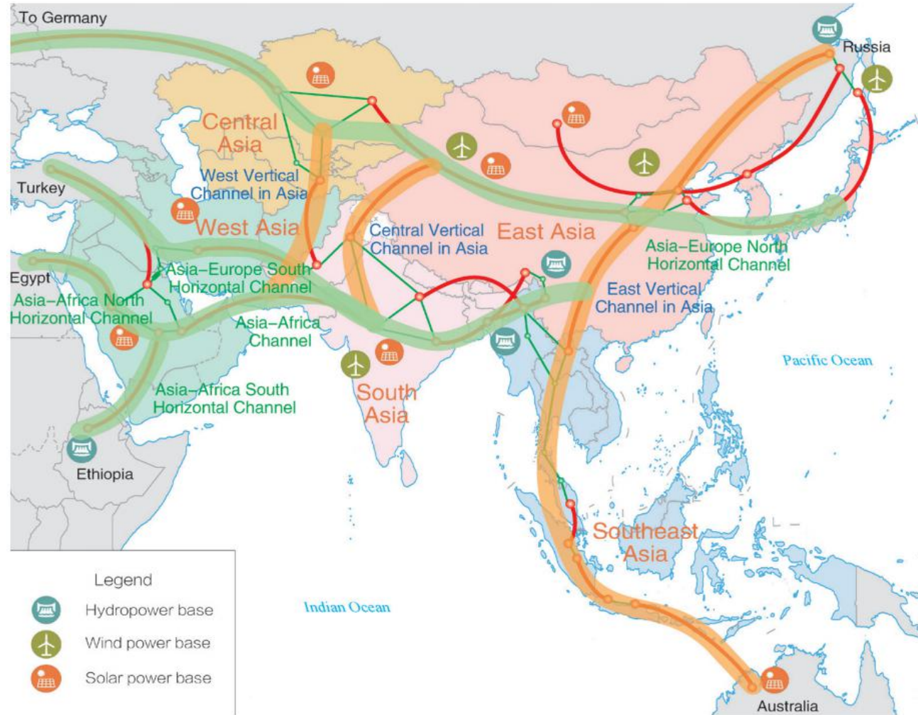
Illustration of Power Grid Interconnection Pattern in Asia
