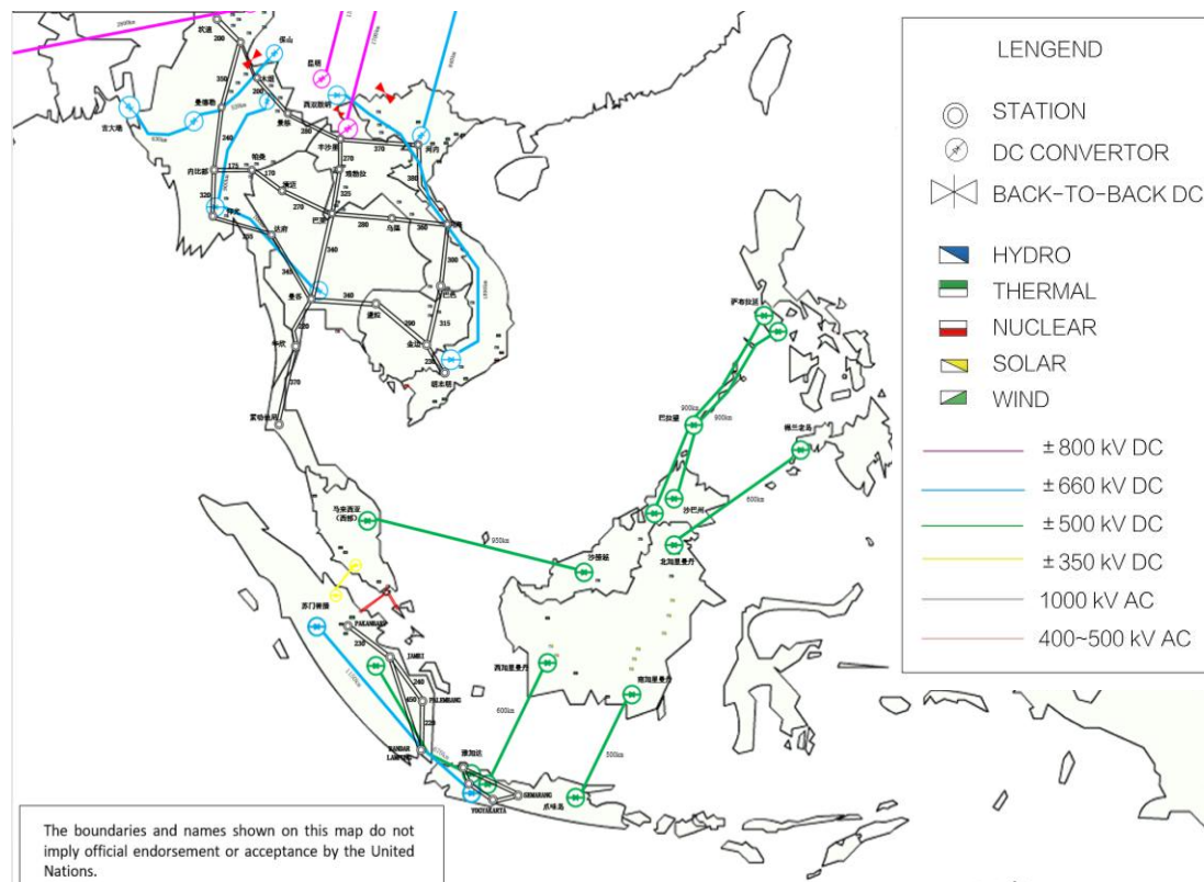
Recommended Backbone Grid
