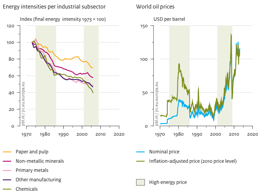
Figure 3.2 Industrial energy intensities and energy prices
