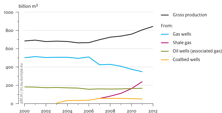
Figure 2.7 Gross natural gas production in the United States
