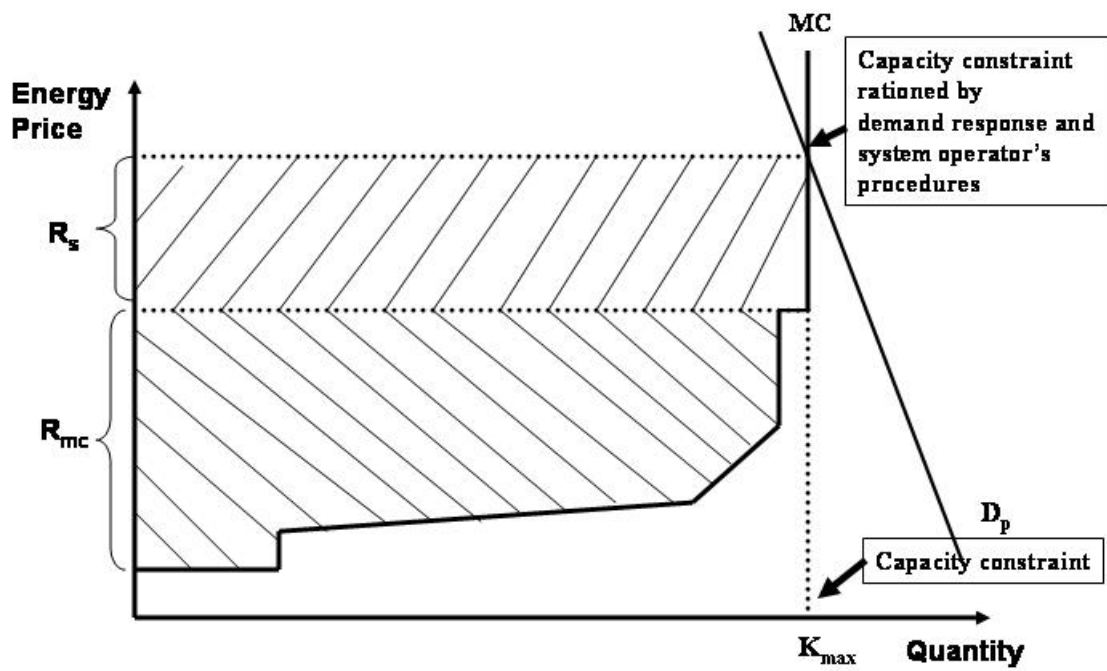
FIGURE 2 PRICING WITH BINDING CAPACITY CONSTRAINTS
