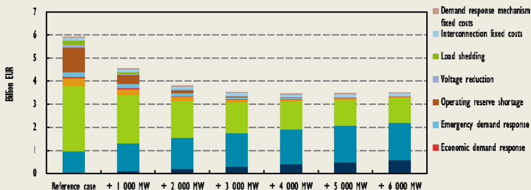
Figure 4.7 • Total reliability costs for different gas-fired capacity additions
