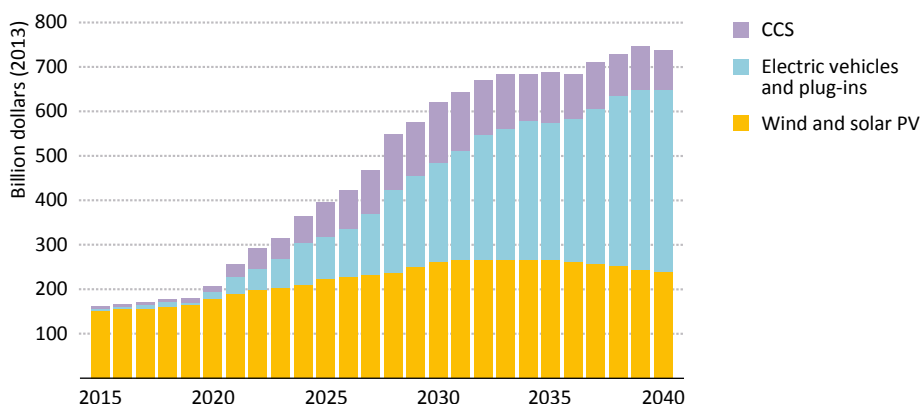
Figure 5.7 ▶ Global investment in variable renewables, CCS and electric vehicles in the 450 Scenario
