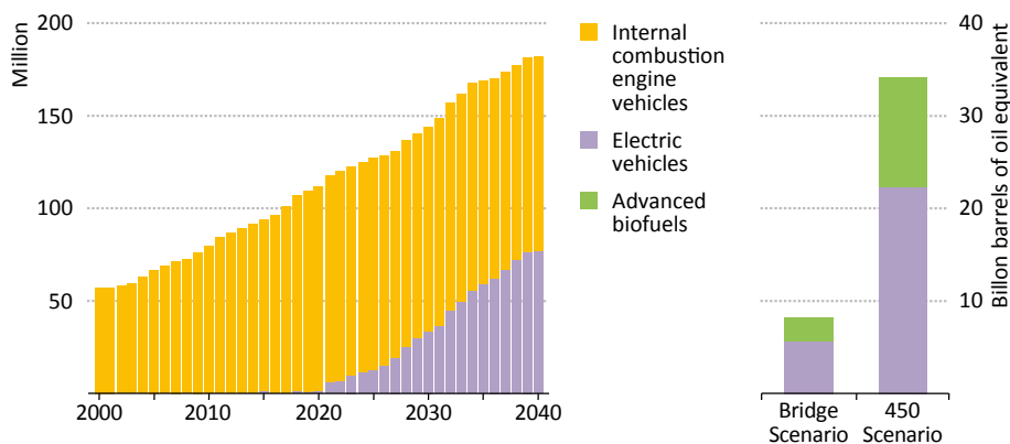
Figure 4.7 ▶ Global light-duty vehicle sales by type in the 450 Scenario (left) and global cumulative oil savings by scenario from electric vehicles and advanced biofuels, 2015-2040 (right)
