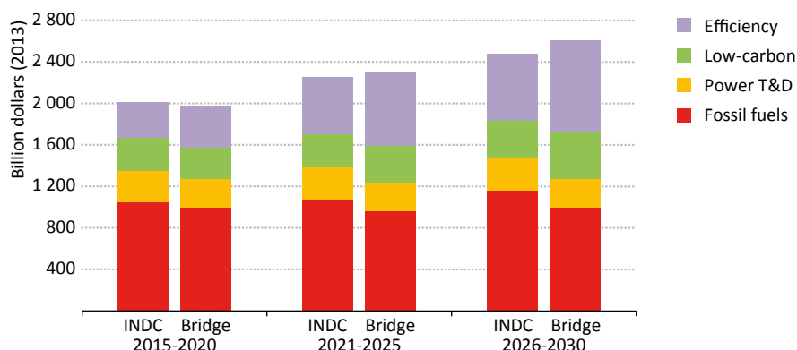
Figure 3.18 ▶ Global average annual investment in the energy sector by type and scenario
